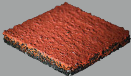
BLACK MAT WITH STRUCTURAL SPRAY 3/8 - 1/2 inch black mat High quality rubber granules Fortified Latex Binder Acrylic structural spray
