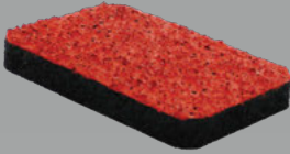
QC 200SS Permeable base mat structural spray system 13 mm, paved in place, base mat 2 coats colorized structural spray
